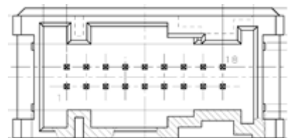
Connector 18 Pin White (2-185529-2)
