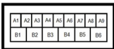
Connector 15 Pin Black (98315-0001)
